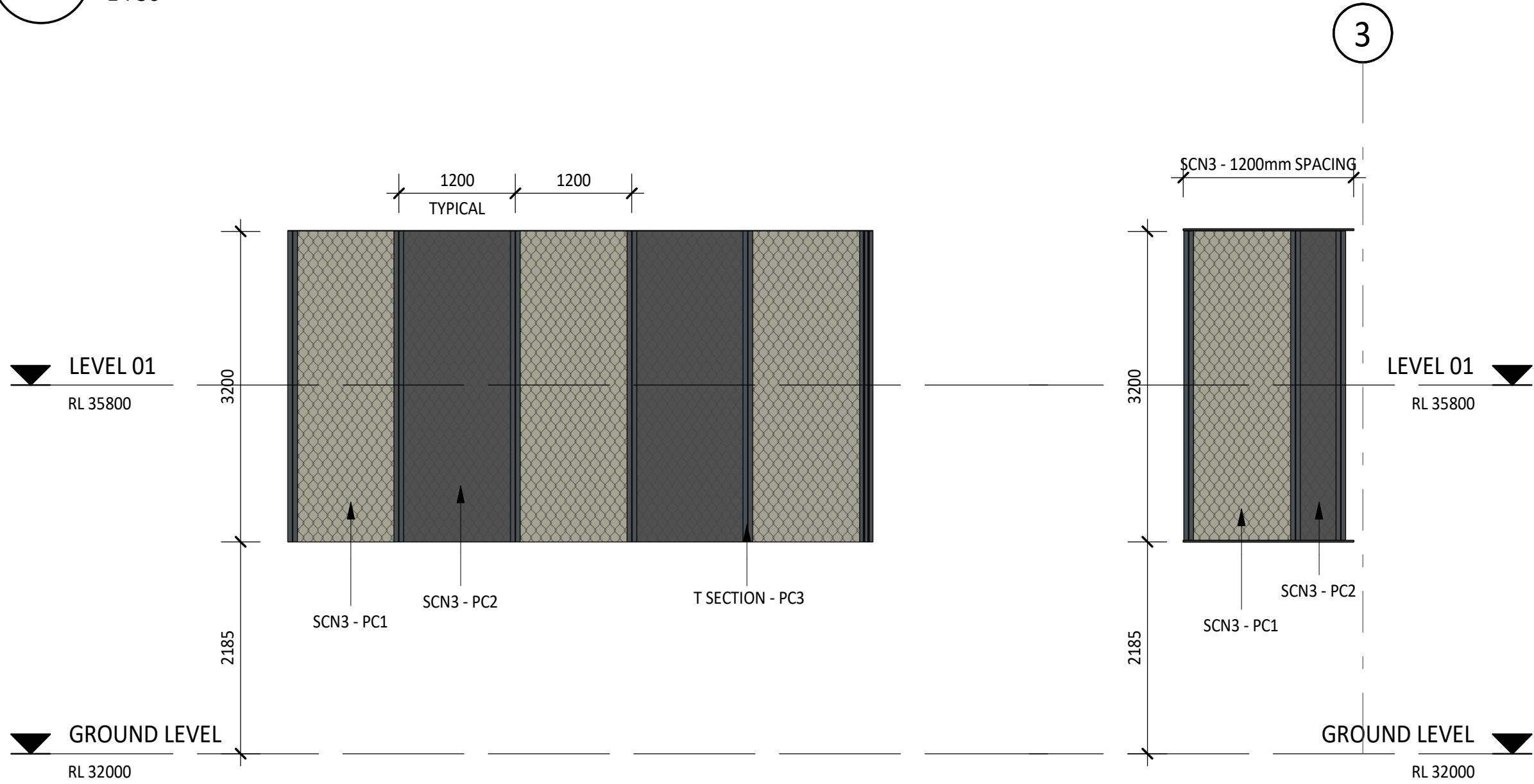
4 WEST SHADE SCREEN 3 ELEVATION 1 : 50
