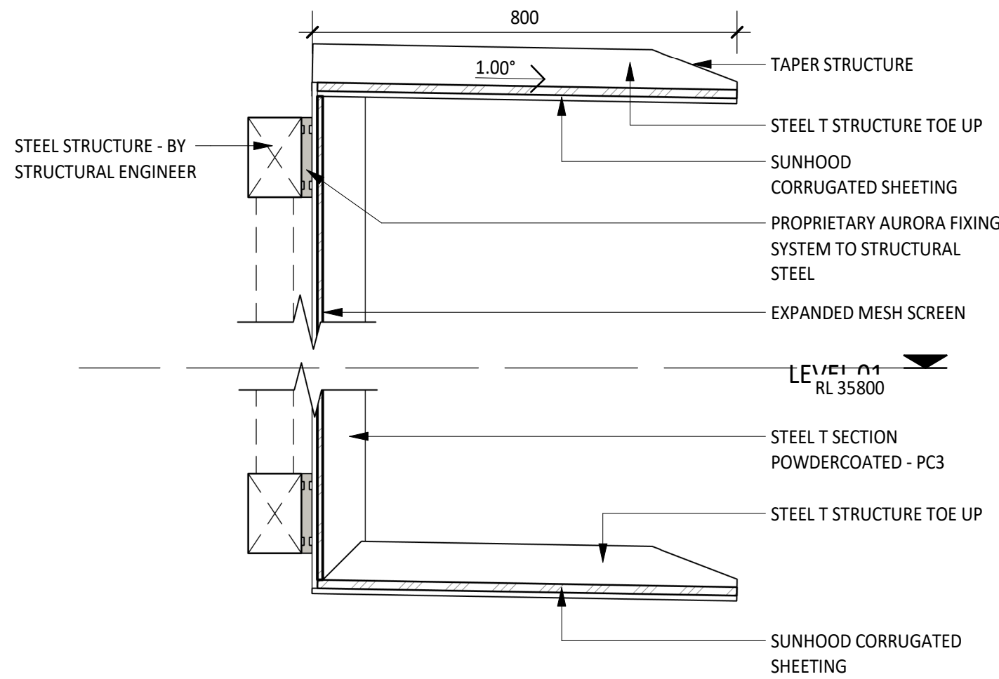
8 SHADE SCREEN SECTION - TYPICAL DETAIL 1 : 10
