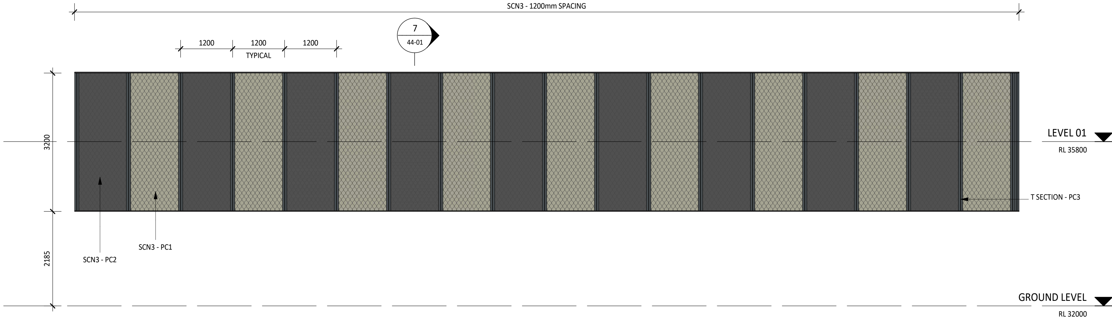
1 WEST SHADE SCREEN 1 1 : 50
