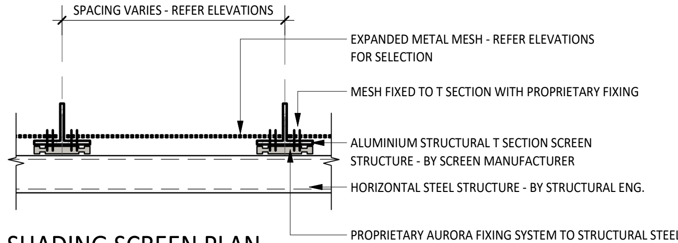
6 SHADING SCREEN PLAN 1 : 10
